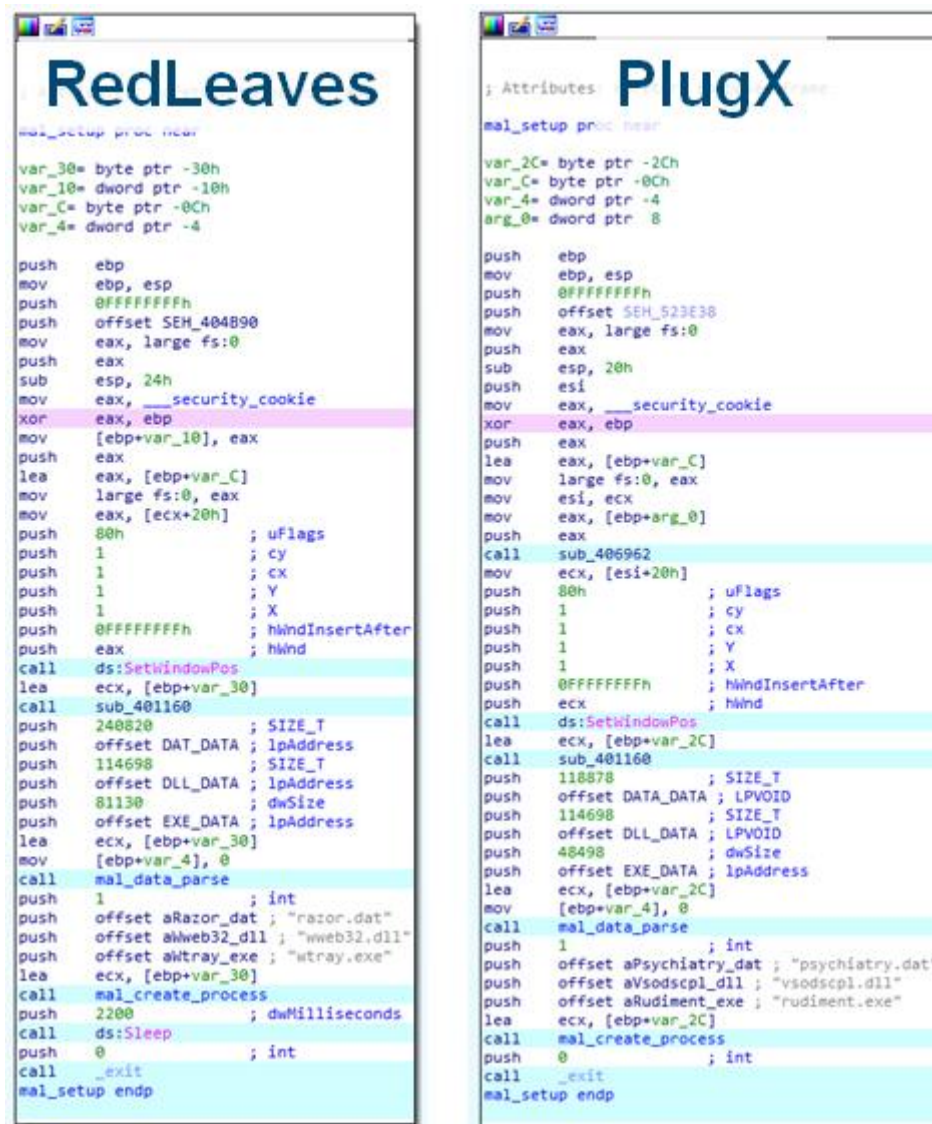
Figure 16: Code comparison between RedLeaves and PlugX 10
